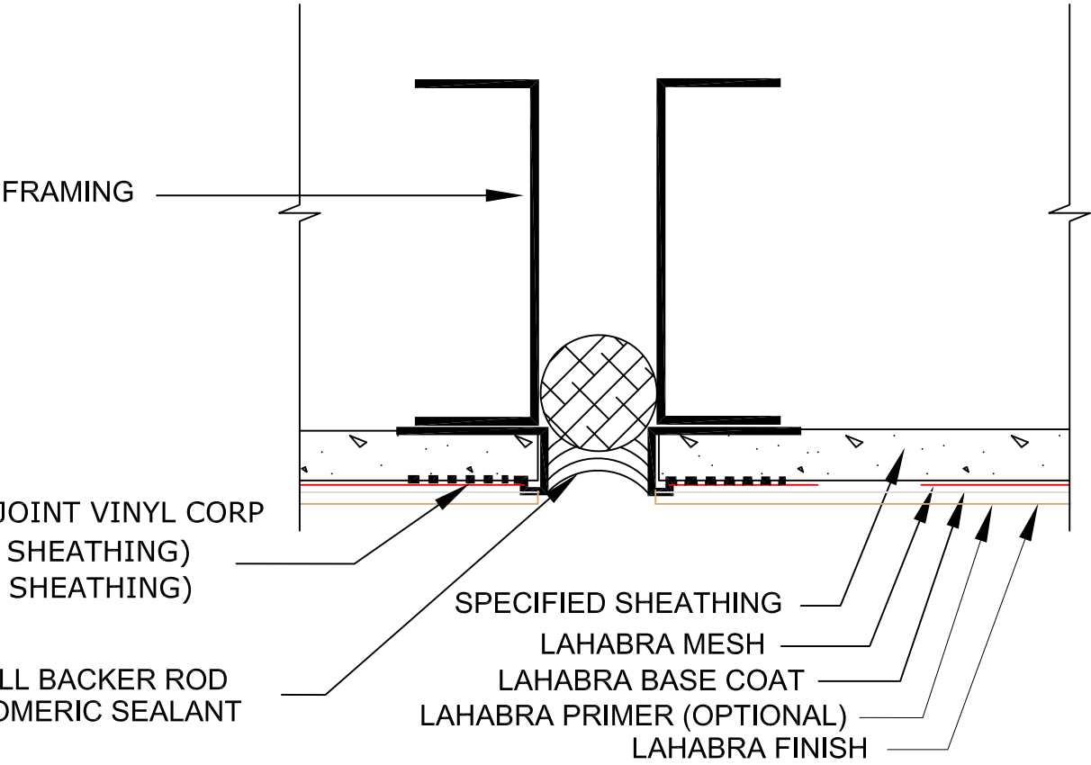
ACF SOFFIT 1.06 EXPANSION JOINT DETAIL
