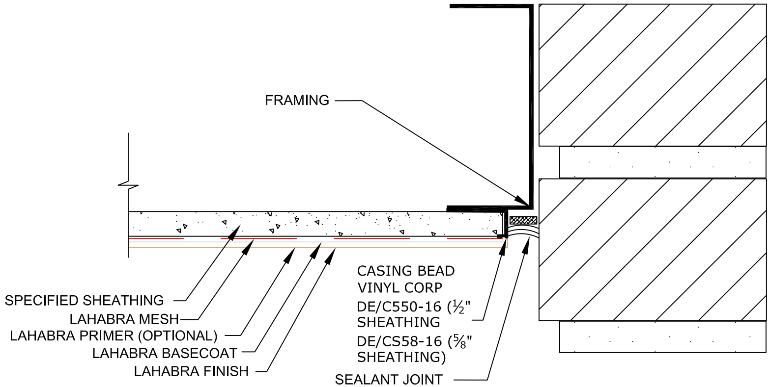
ACF SOFFIT 1.01 EDGE TERMINATION DETAIL
